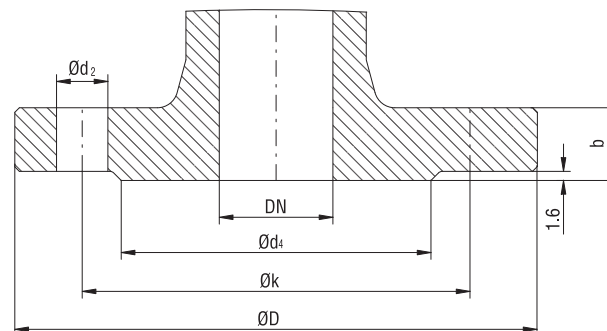
CLASS 150,300,600
